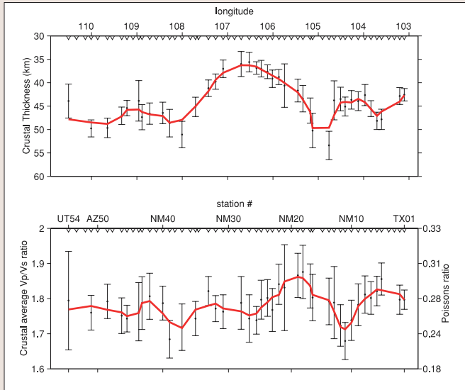
Figure 4. Crustal thickness and average V_p/V_s ratios determined from moveout analysis of primary and reverberated P-to-S converted modes. The red line shows a three-point weighted mean.
