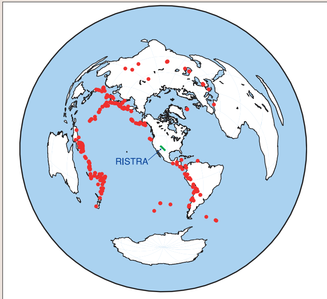
Figure 2. Global distribution of the 285 earthquakes (red points) with body-wave magnitude > 5.6, recorded during the RISTRA network deployment, which have suitable offsets for calculating the 8361 receiver functions used in this study. We use teleseisms from epicentral distances of 25-105°, which have incident angles ranging from approximately 40-15° at the base of the crust. The RISTRA seismometer deployment (green) is a great-circle swath.
